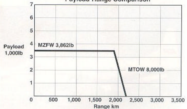
Cessna 208B Super Cargomaster Payload-Range Comparison
