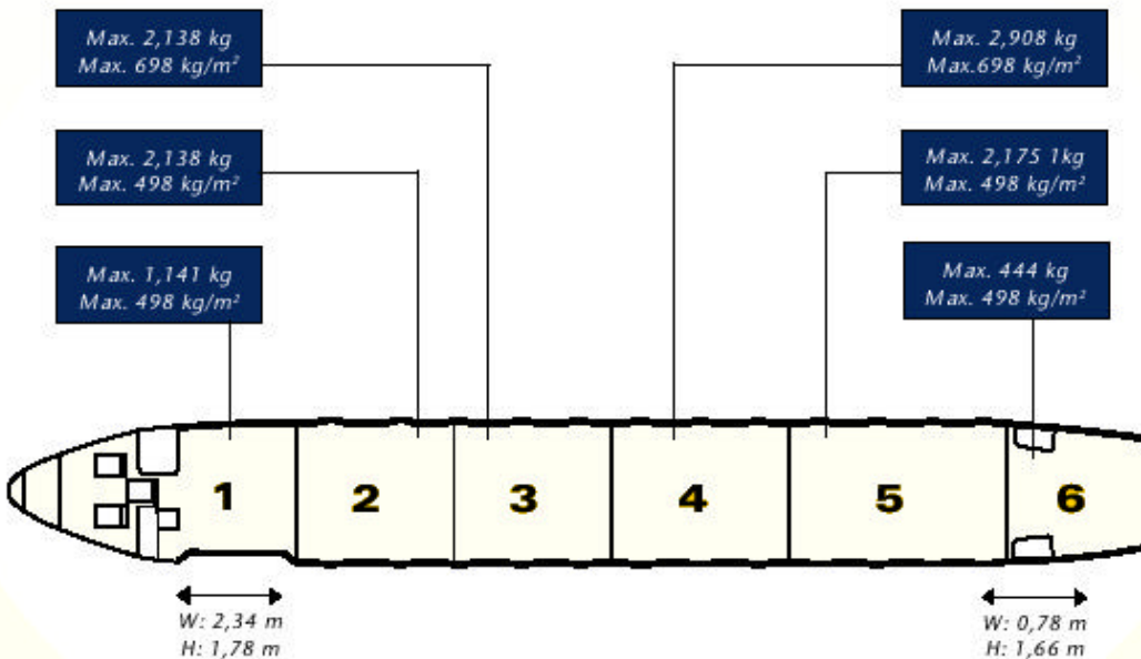
Cargo Door Openings Fokker F27-600
